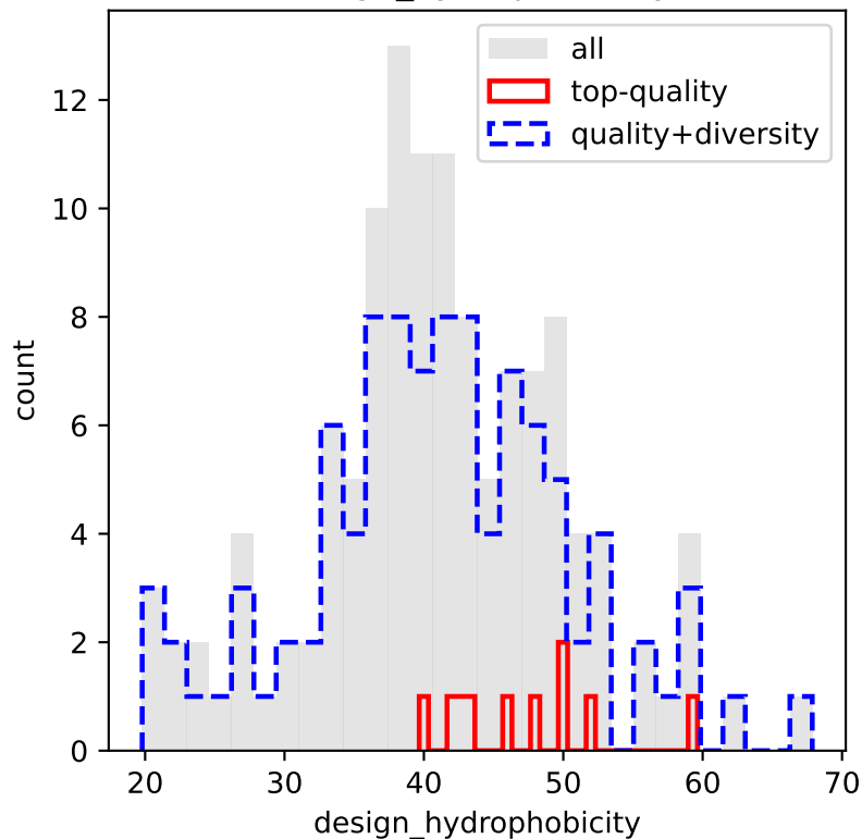
design_hydrophobicity
