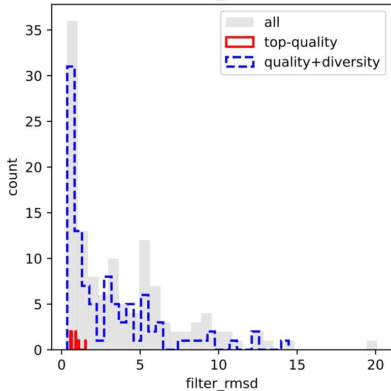
filter_rmsd
