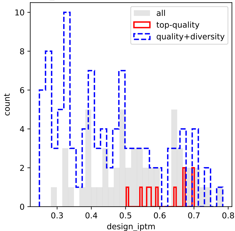
design_ipmtm (Designs passing RMSD threshold)
