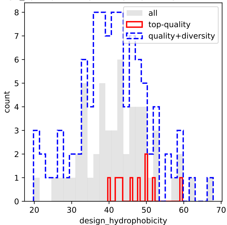
design_hydrophobicity (Designs passing RMSD thres
