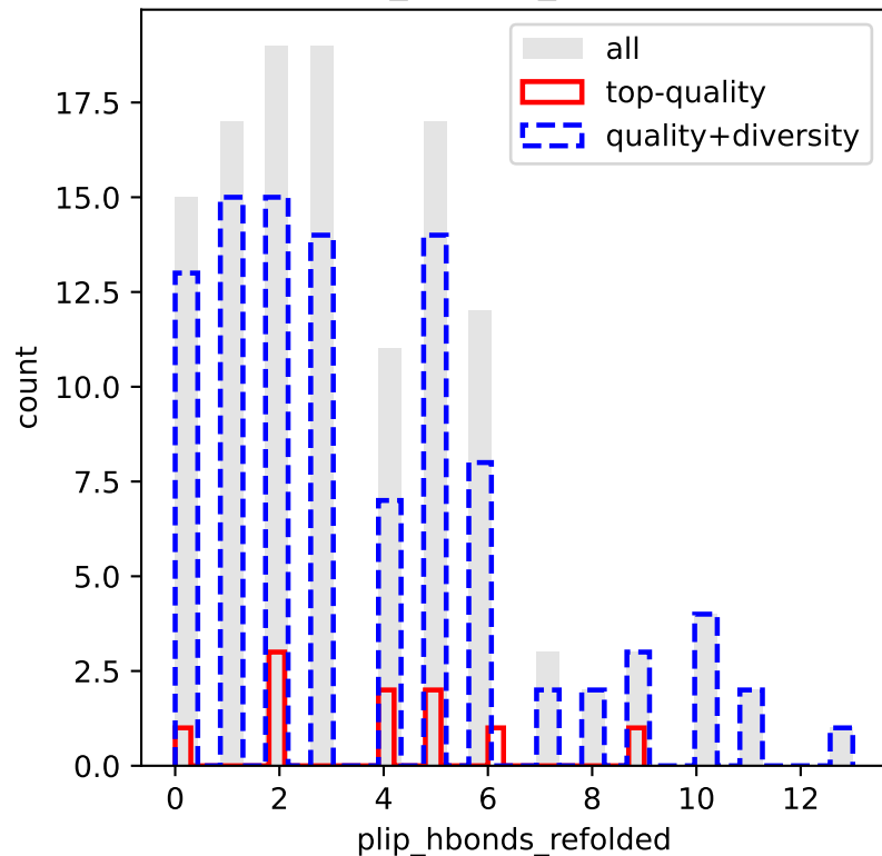
plip_hbonds_refolded
