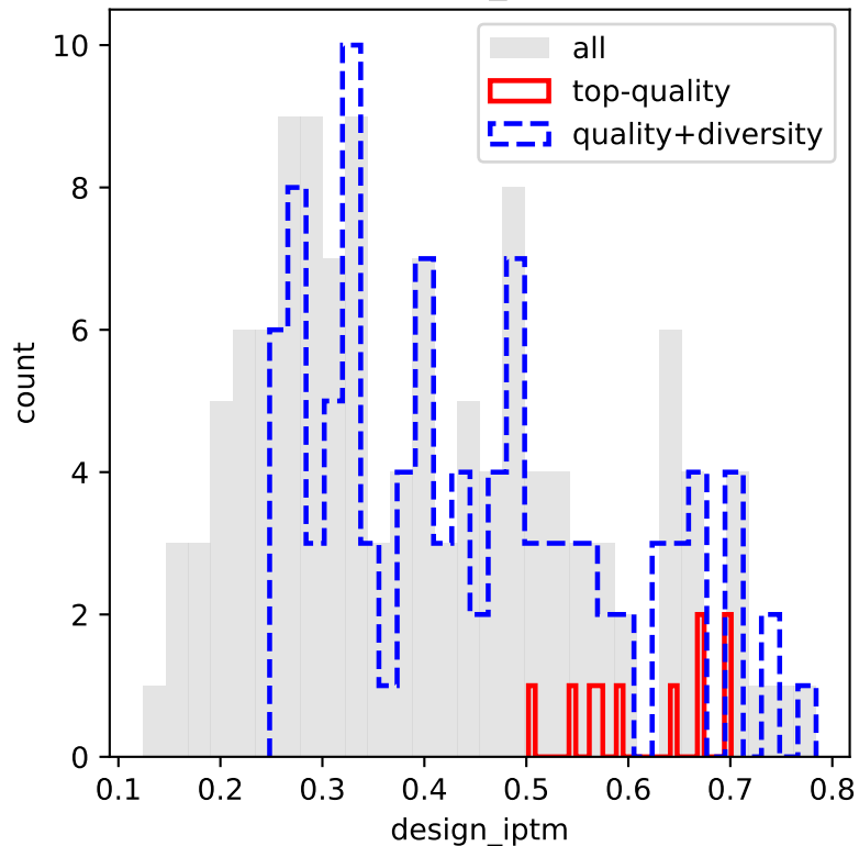
design_ipmtm
