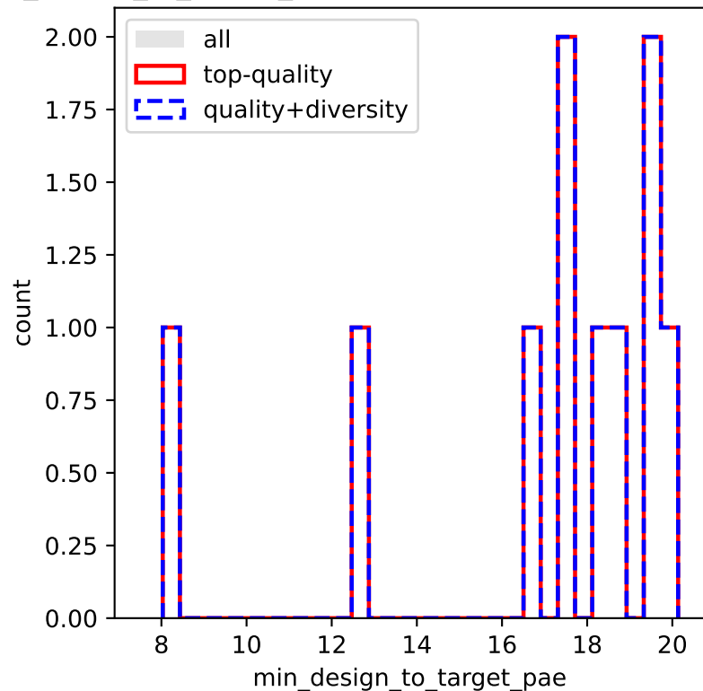
min_design_to_target_pae (Designs passing RMSD th
