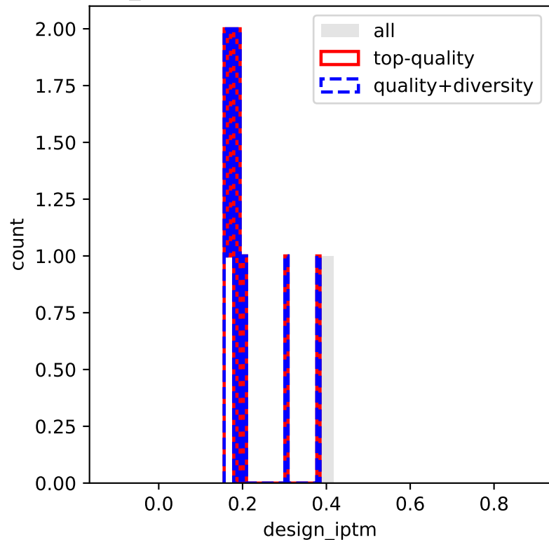
design_iptm (Designs passing RMSD threshold)
