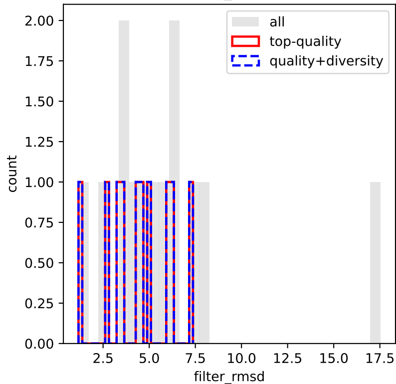
filter_rmsd
