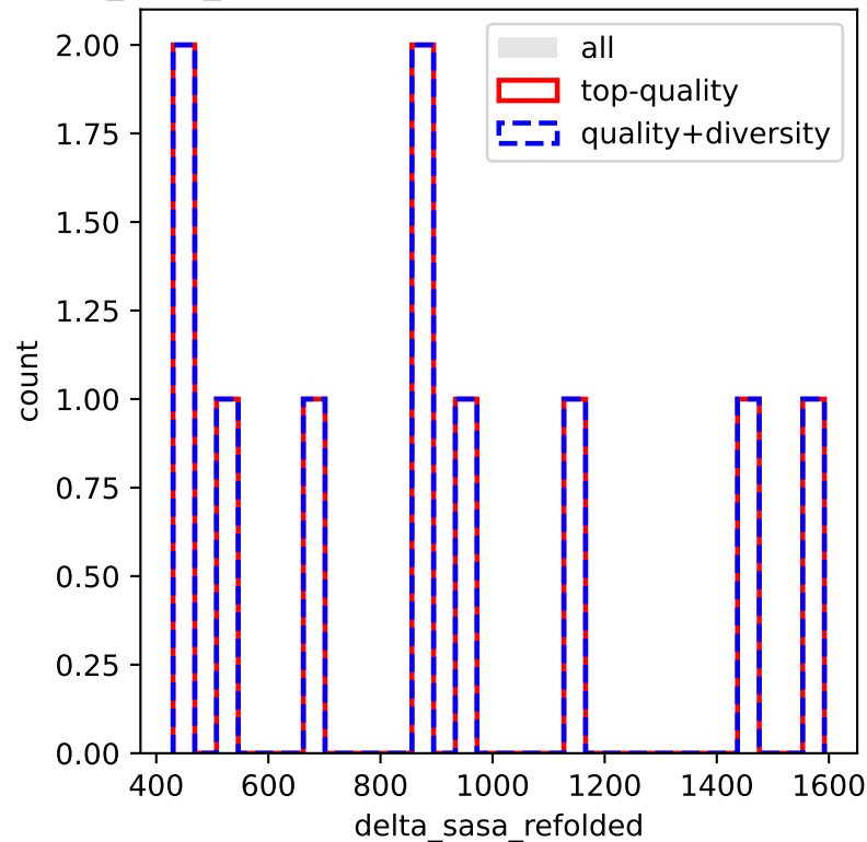
delta_sasa_refolded (Designs passing RMSD thresh
