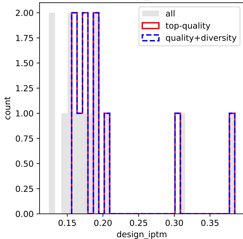
design_iptm
