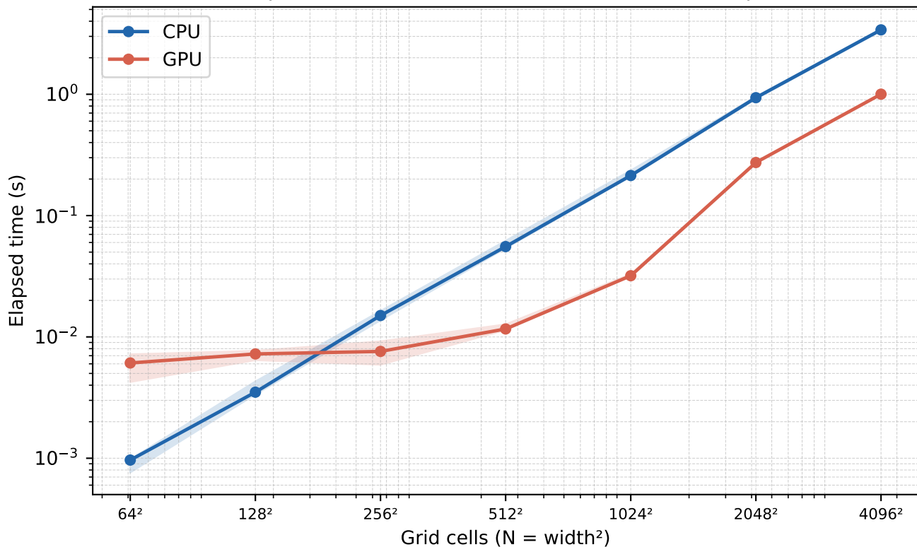
Experiment 1a — Wall-clock time for 500 steps
