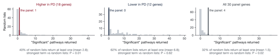
Figure 9: Over-representation with the 5,622 measured genes as background and Benjamini-Hochberg correction. (a) Terms for the lower, higher and full panel. (b) The four significant terms and the five genes that carry them. (c) The same settings applied to 100 random gene lists of each size.
