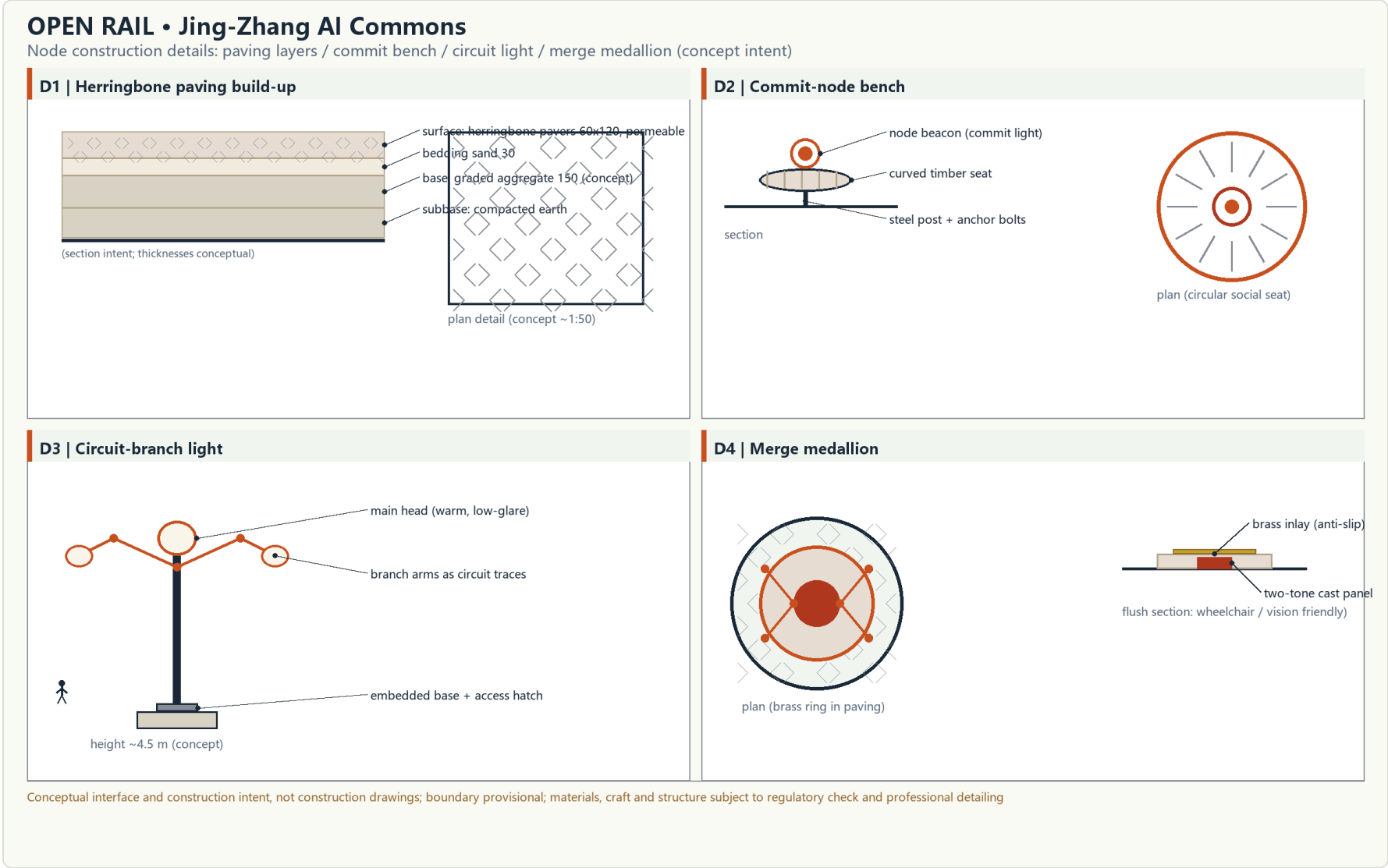
Fig.3f | Node construction details: paving / bench / light / medallion (intent, not construction drawings)
