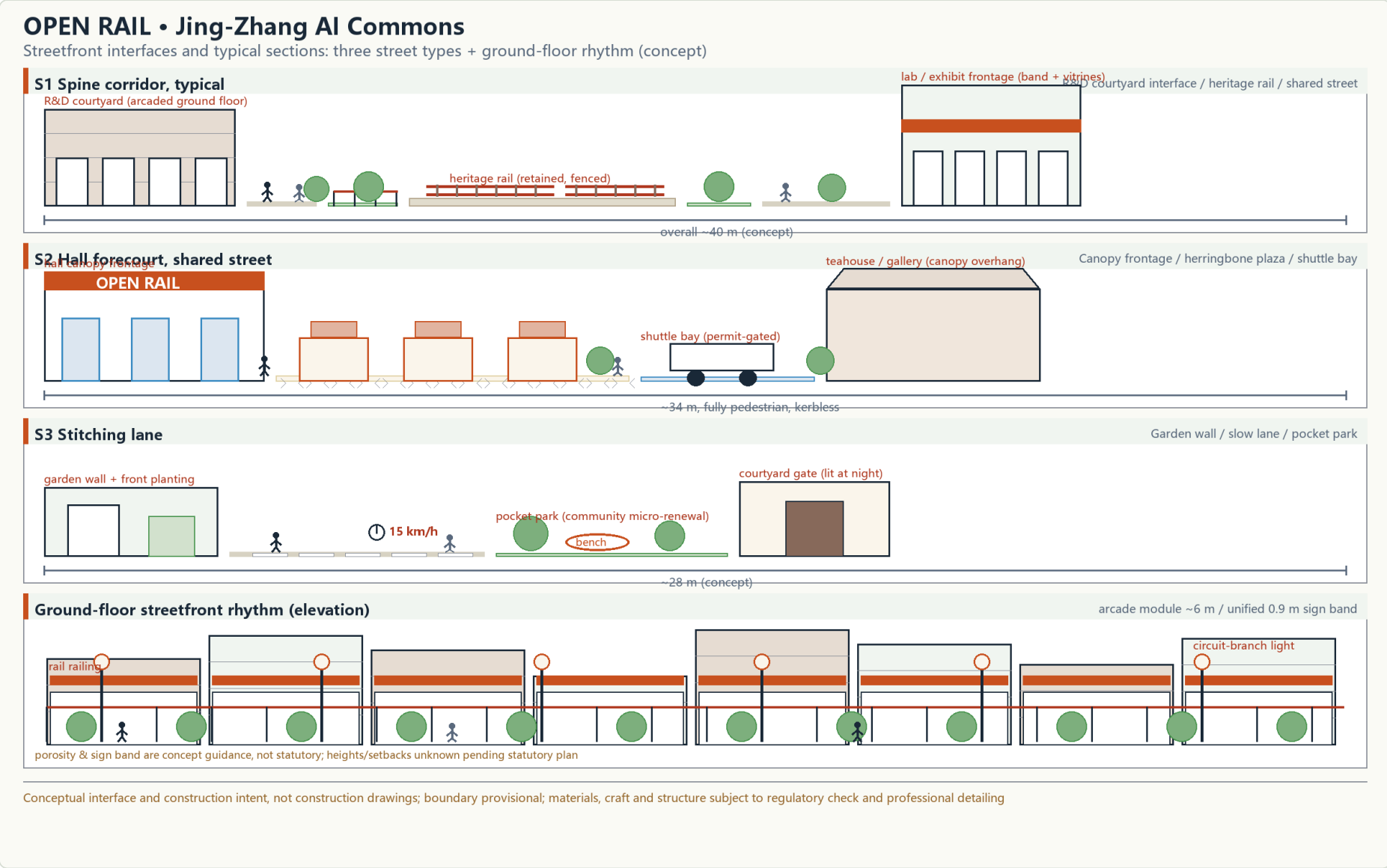
Fig.3e | Streetfront interfaces & typical sections (S1 corridor / S2 forecourt / S3 lane + ground-floor rhythm; concept)
