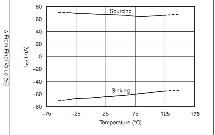
Figure 40. Short-Circuit Current vs Temperature
