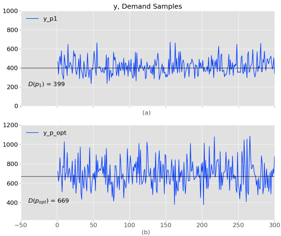
Figure 1: Each plot shows demand samples over 300 periods ( a = 4000 , v = 1.8 , CV_d = 0.2 ) at two price levels: (a) p_1 = \$3.6 and (b) p_{opt} = \$2.7 .
