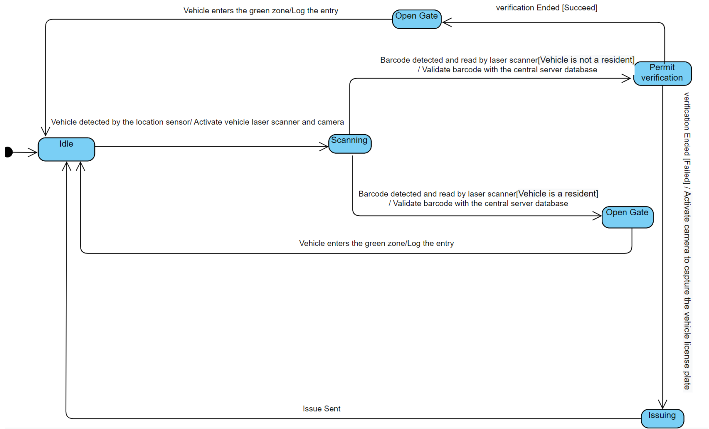
5.1. Entry Statechart
