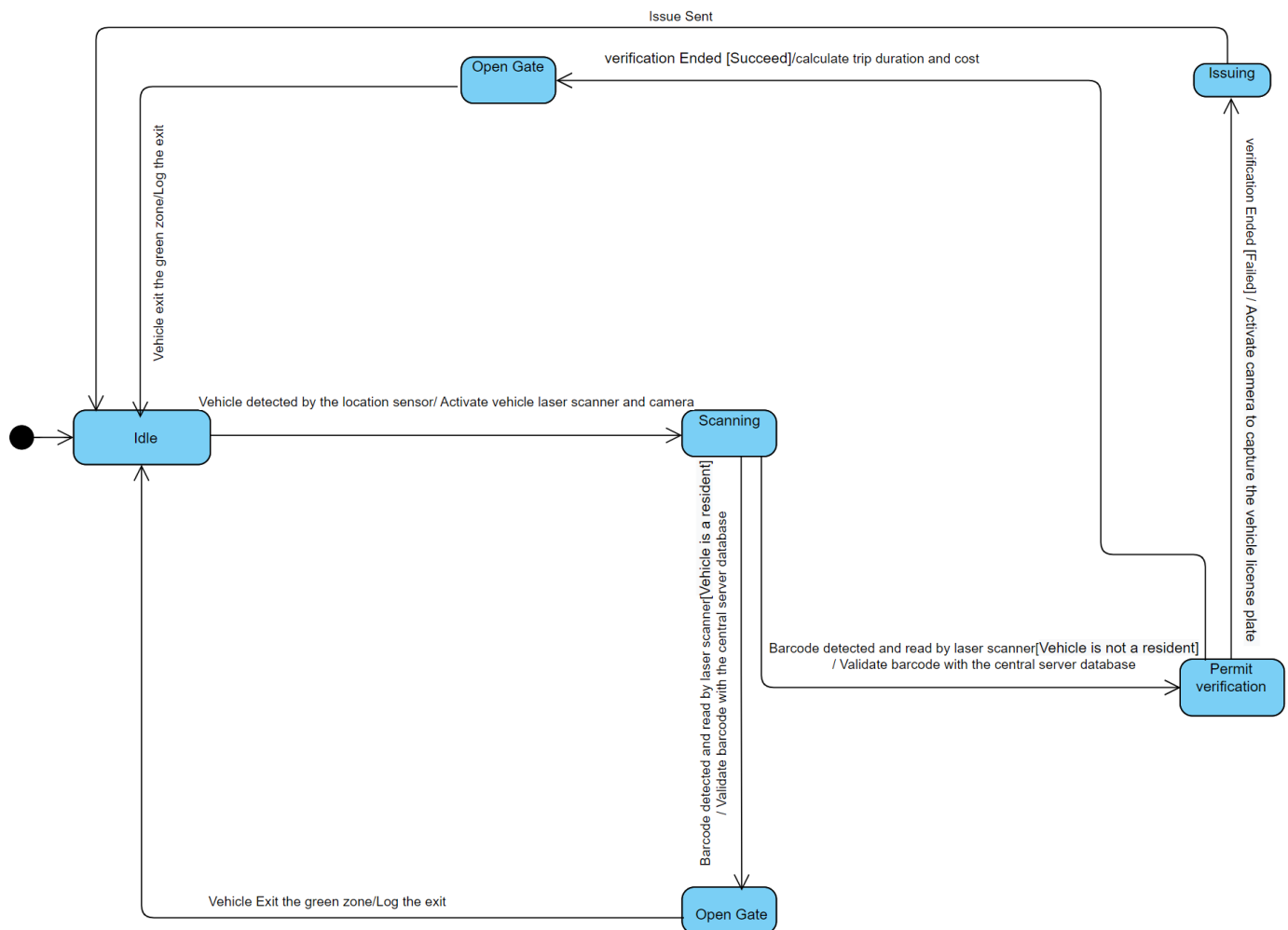
5.2. Exit Statechart
