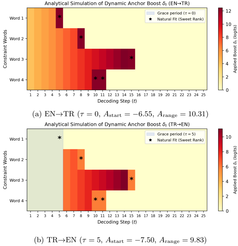
Fig. 3. Dynamic anchor schedule for each direction. Colour intensity indicates applied logit boost \delta_t . The grace period (zero boost), sweet-rank windows (light buffer), and full anchor pressure are distinguishable. The EN→TR direction applies pressure from step 1; TR→EN waits five steps.
