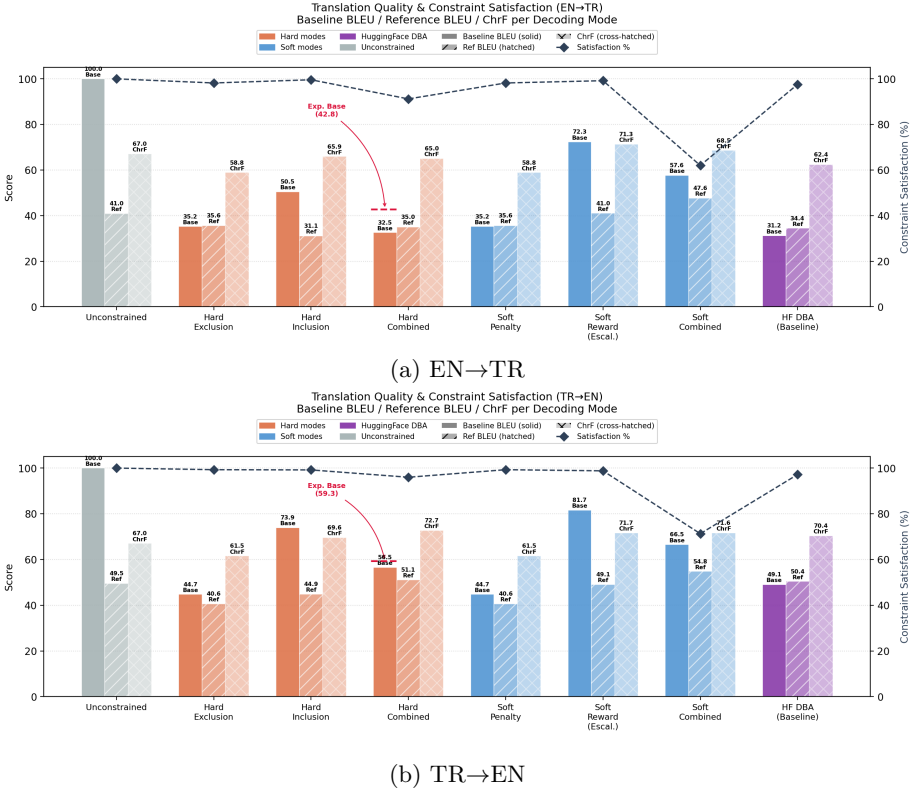
Fig. 2. Translation quality (Baseline BLEU / Reference BLEU / ChrF) and constraint satisfaction per decoding mode, for both translation directions.
