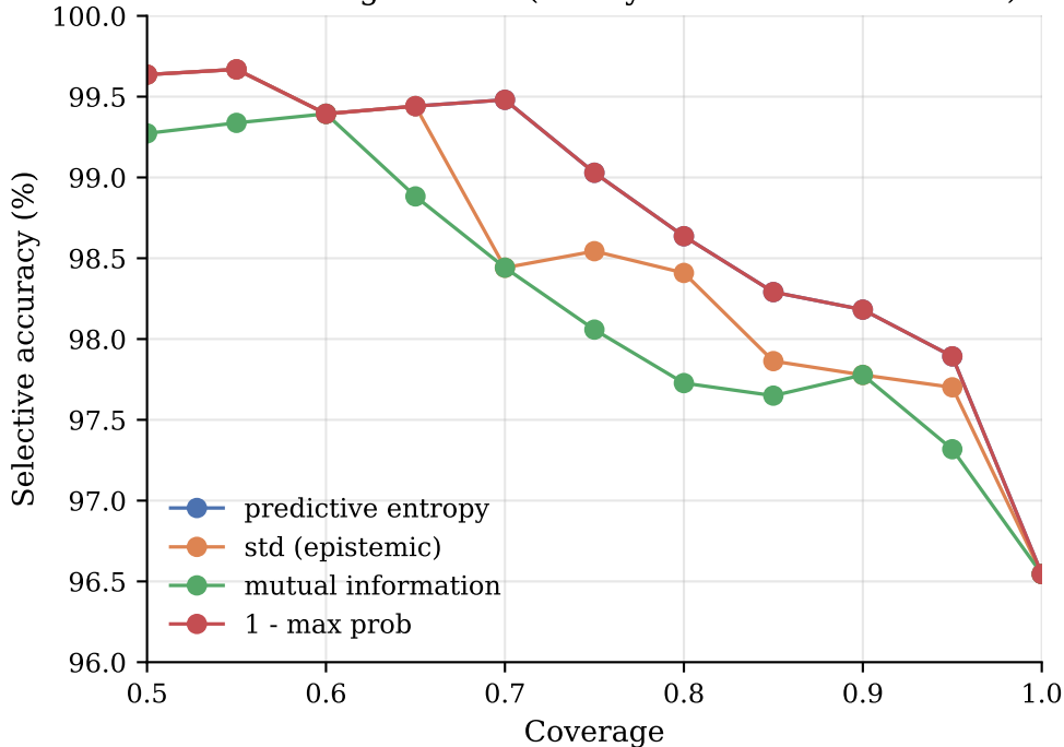
Risk-coverage curves (binary ensemble of 6 models)
