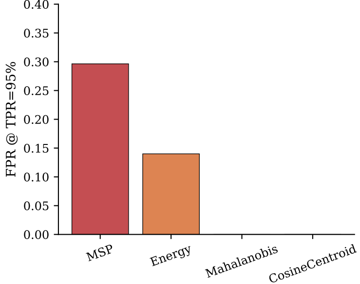
OOD false-positive rate (lower better)
