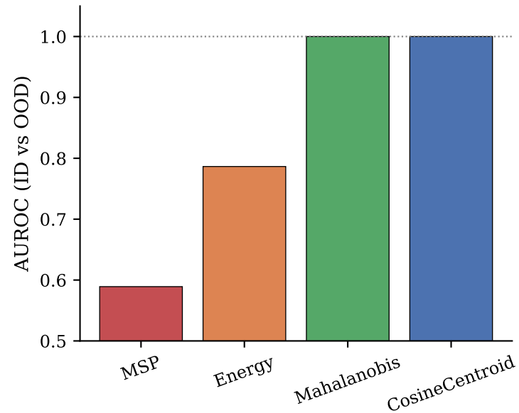
OOD detection AUROC (higher better)
