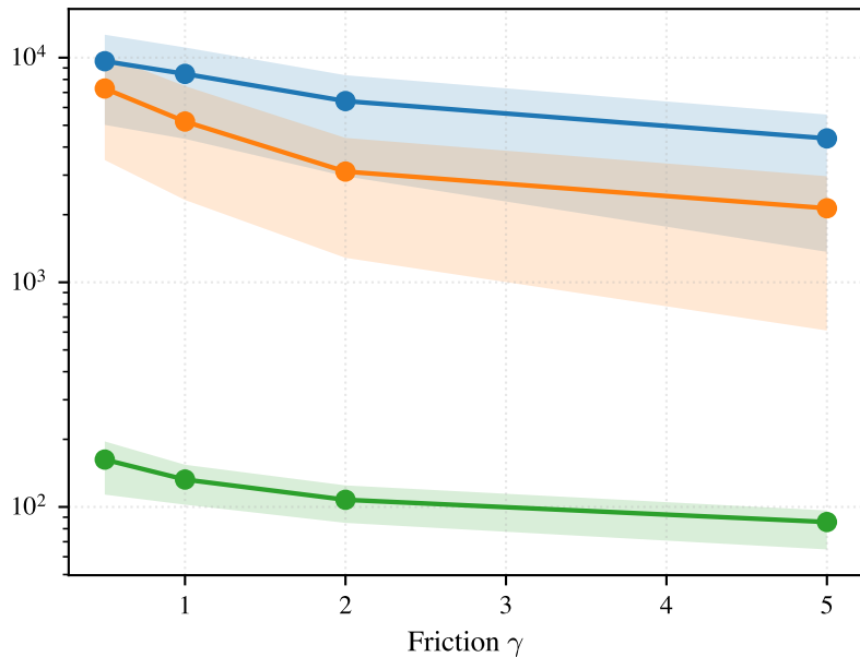
Mean ESS (mean over \eta, d ; IQR band)
