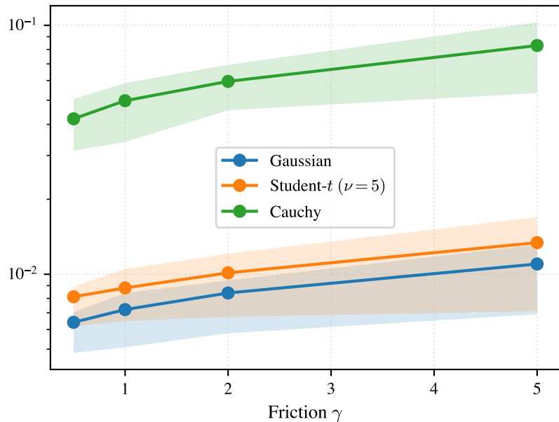
KS (mean over \eta, d ; IQR band)
