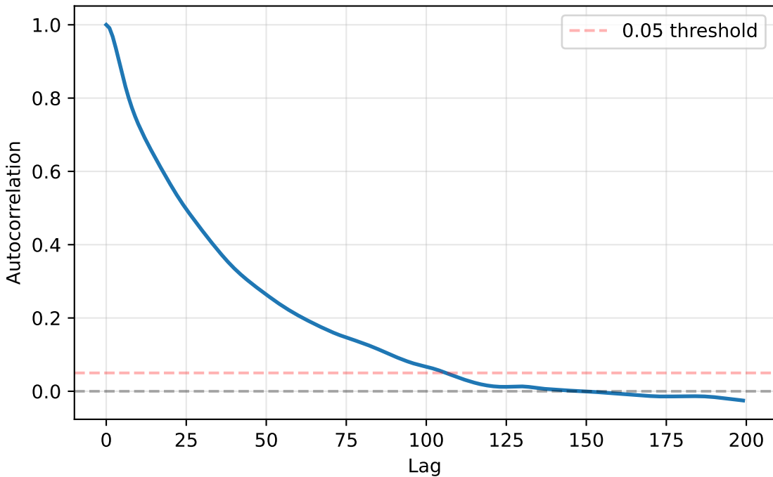
ACF - Dimension 0
