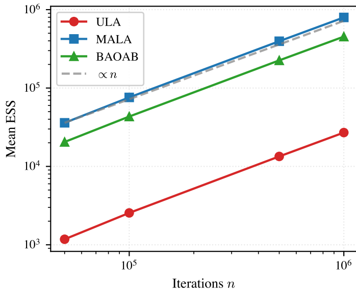
Gaussian
