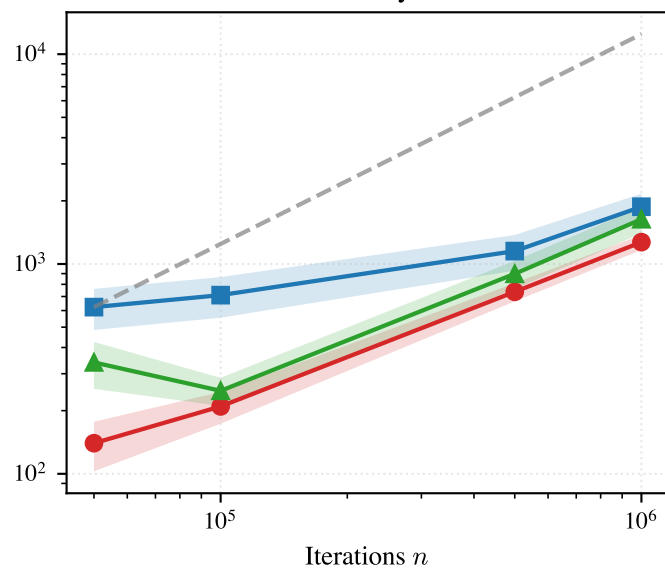
Cauchy
