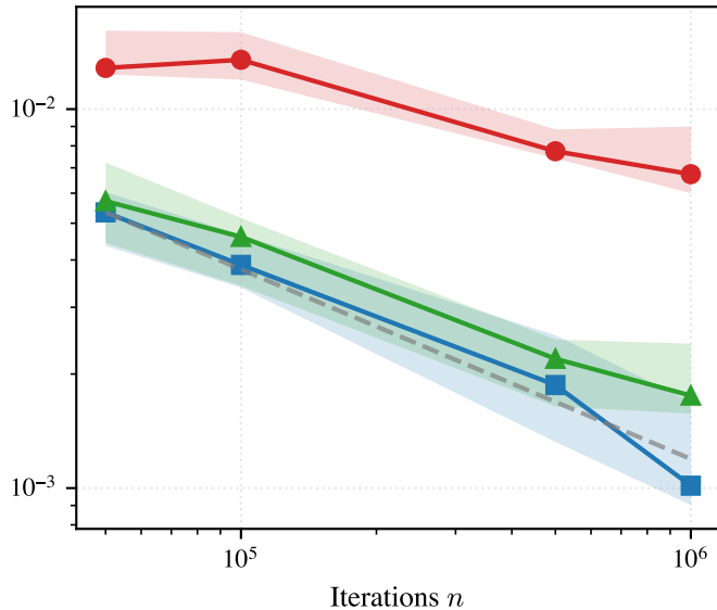
Student- t ( \nu = 5 )
