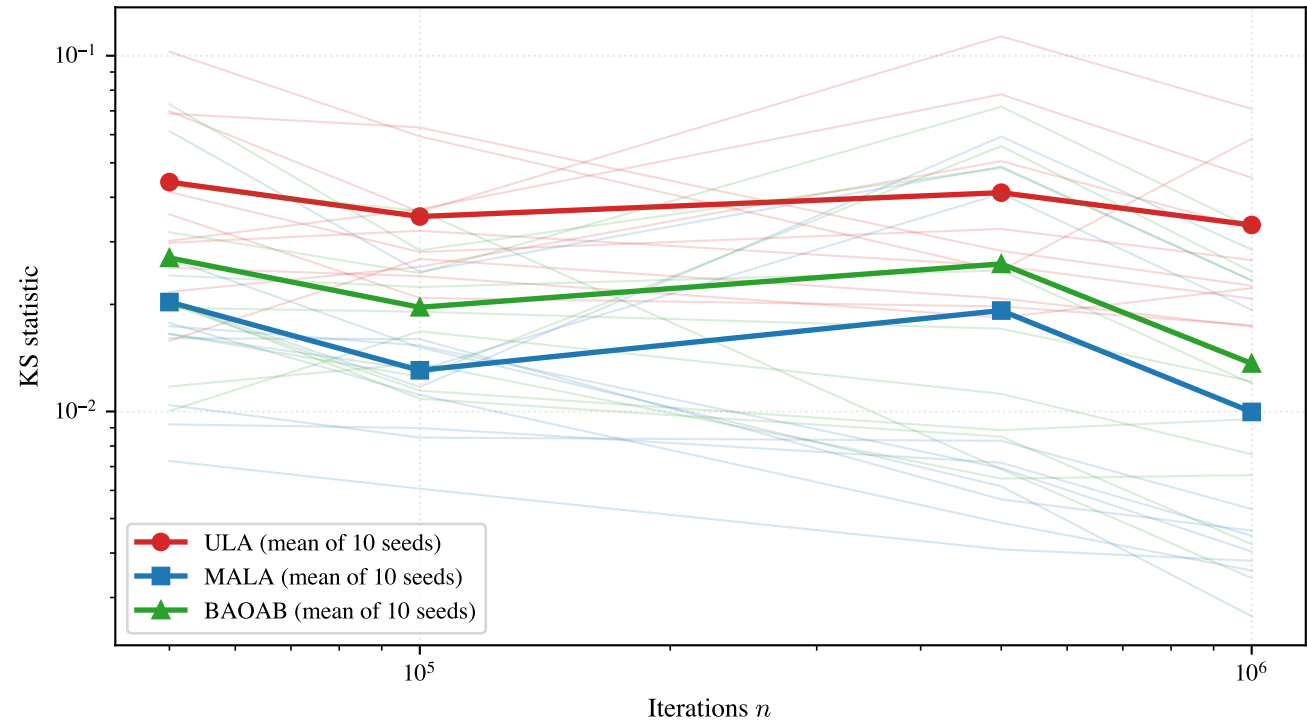
Per-seed KS trajectories on Cauchy
