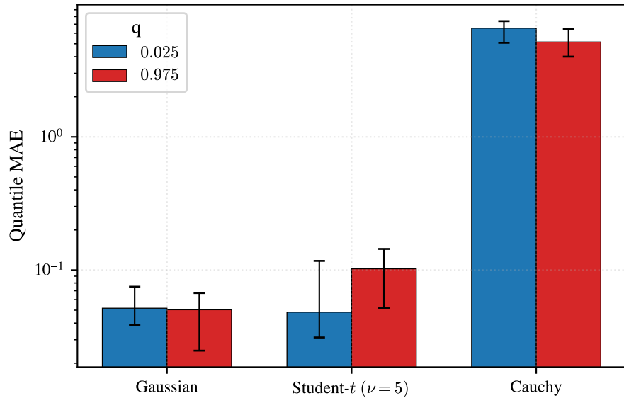
ULA quantile error at \eta = 0.1 , d = 1
