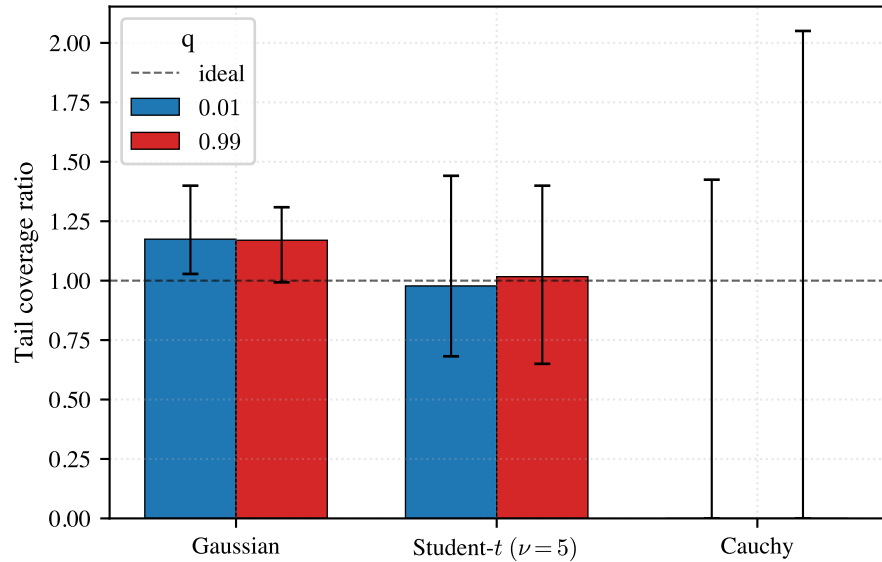
ULA tail coverage at \eta = 0.1 , d = 1
