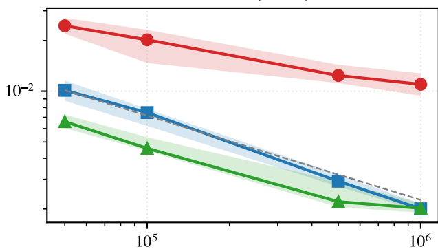
Banana ( b = 0.03 )
