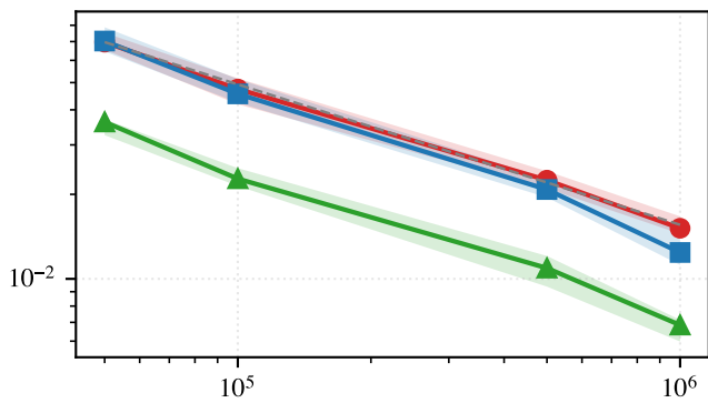
Funnel ( \sigma_v = 2 )
