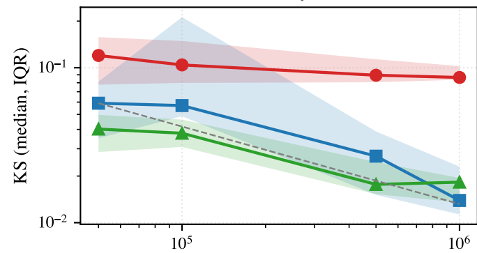
Mixture ( a = 6 )
