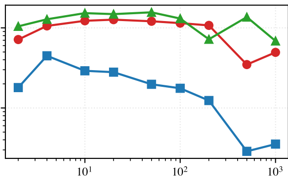
Double well ( \beta = 16 )
