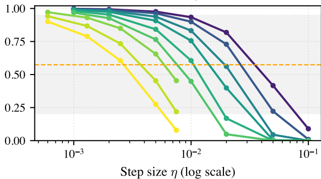
Double well ( \beta = 16 )
