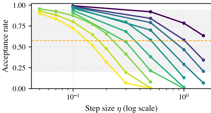
Cauchy
