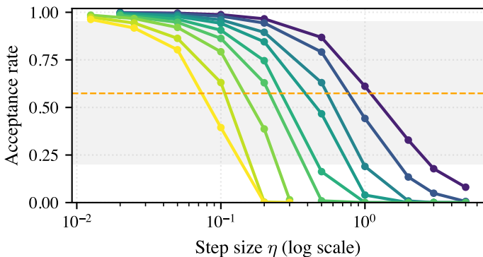
Funnel ( \sigma_v = 2 )
