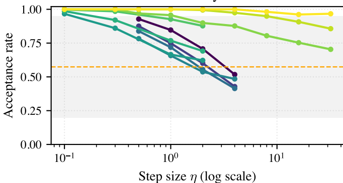
Banana ( b = 0.03 )
