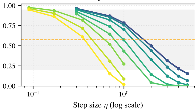
Mixture ( a = 6 )
