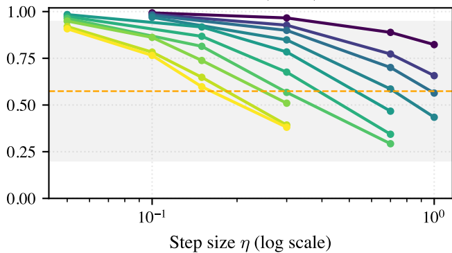
Anisotropic ( \kappa = 1000 )
