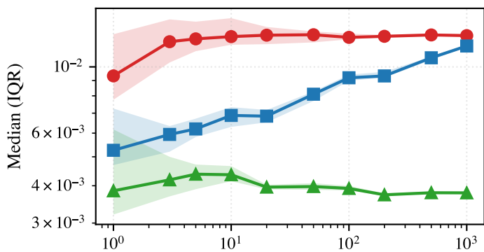
Gaussian: KS
