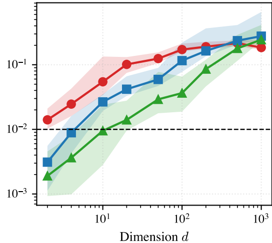
Funnel ( \sigma_v = 2 )
