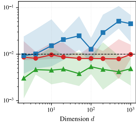
Mixture ( a = 6 )
