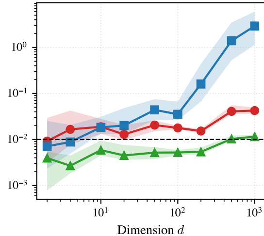
Banana ( b = 0.03 )
