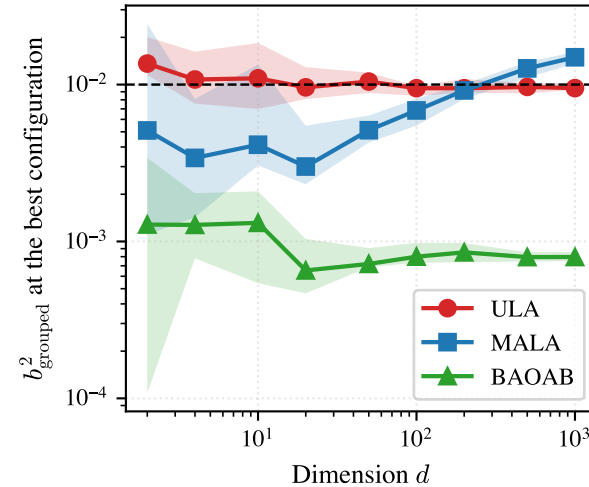
Anisotropic ( \kappa = 1000 )
