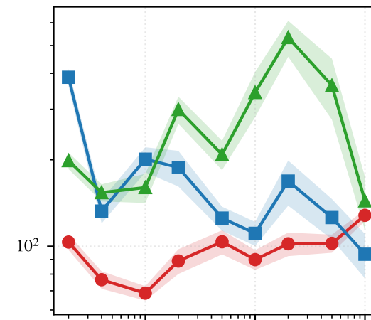
Funnel ( \sigma_v = 2 )
