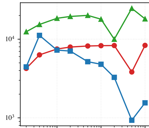
Mixture ( a = 6 )
