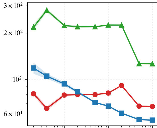
Banana ( b = 0.03 )
