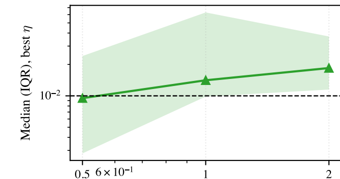
Funnel ( \sigma_v = 2 ): b^2
