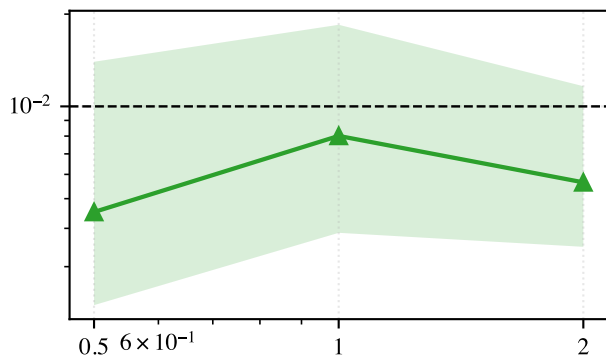
Double well ( \beta = 16 ): b^2
