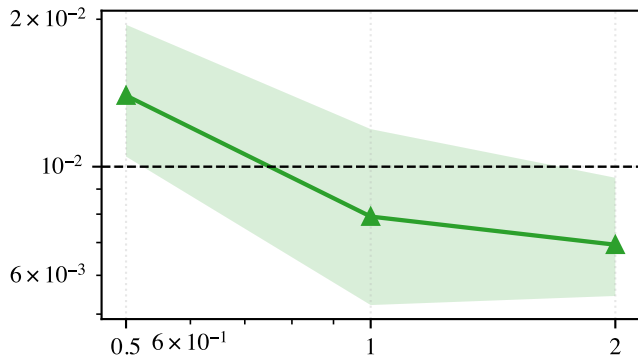
Double well ( \beta = 16 ): b^2
