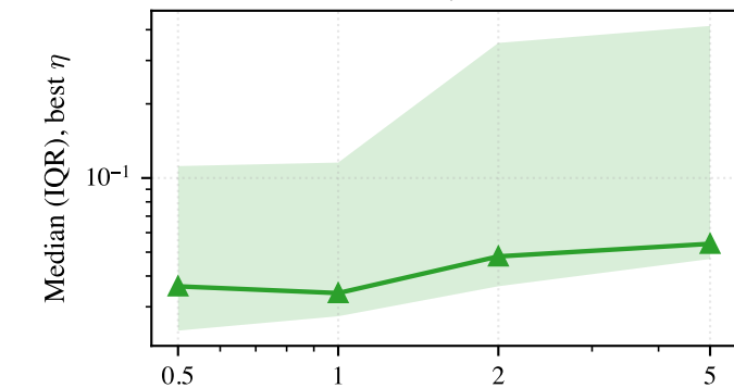
Banana ( b = 0.03 ): b^2
