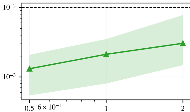
Mixture ( a = 6 ): b^2
