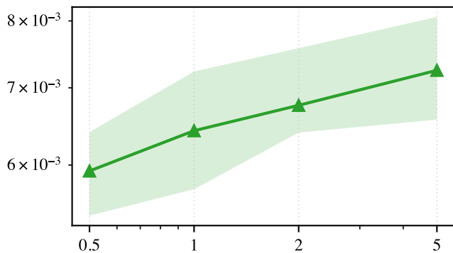
Anisotropic ( \kappa = 1000 ): b^2
