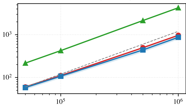
Funnel ( \sigma_v = 2 )
