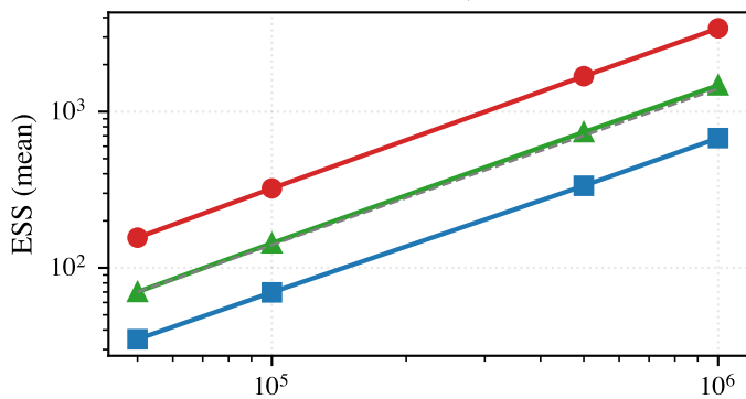
Double well ( \beta = 16 )
