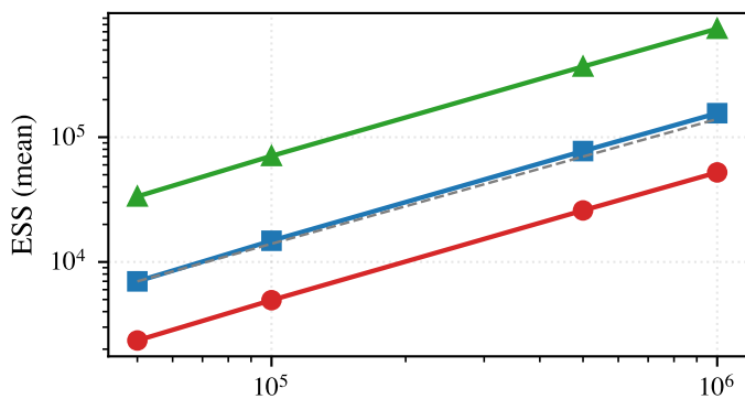
Cauchy
