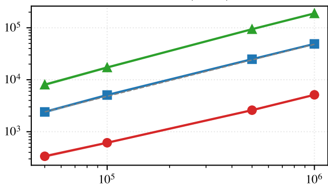
Banana ( b = 0.03 )
