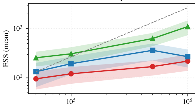
Mixture ( a = 6 )
