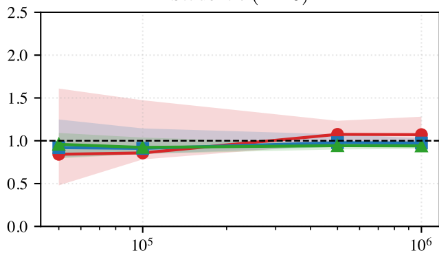
Banana ( b = 0.03 )
