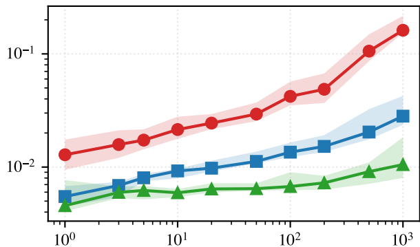
Anisotropic ( \kappa = 1000 )
