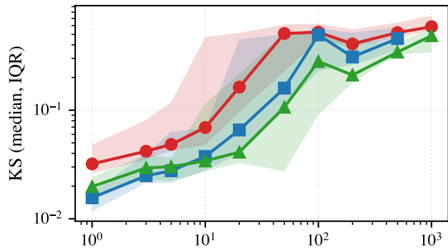
Banana ( b = 0.03 )
