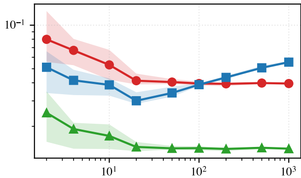
Mixture ( a = 6 )
