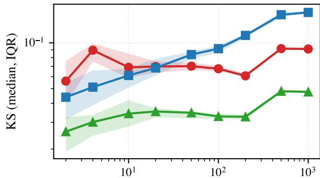
Funnel ( \sigma_v = 2 )
