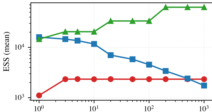
Cauchy
