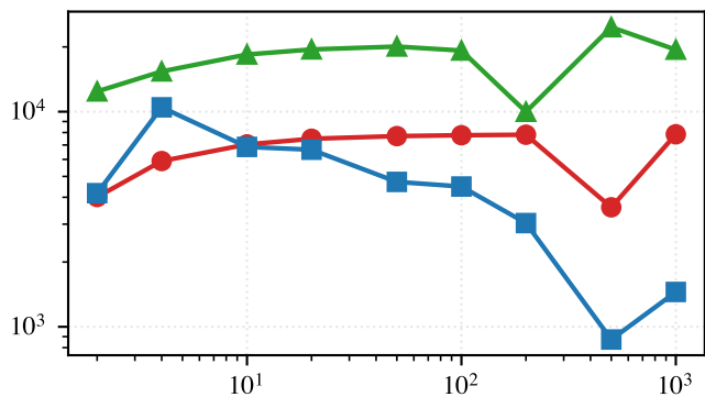
Double well ( \beta = 16 )
