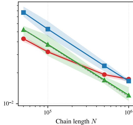
Double well ( \beta = 16 )
