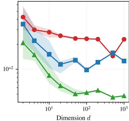
Mixture ( a = 6 )
