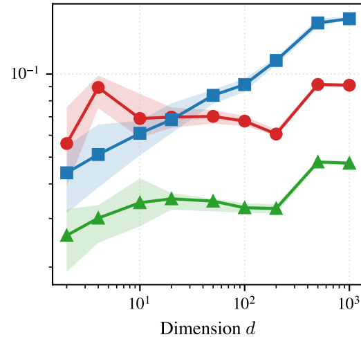
Banana ( b = 0.03 )
