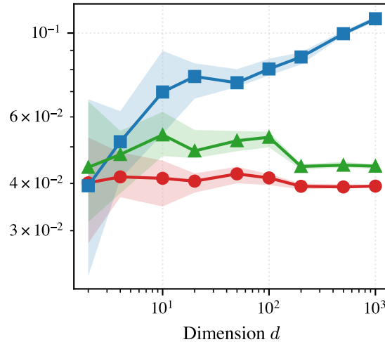
Double well ( \beta = 16 )
