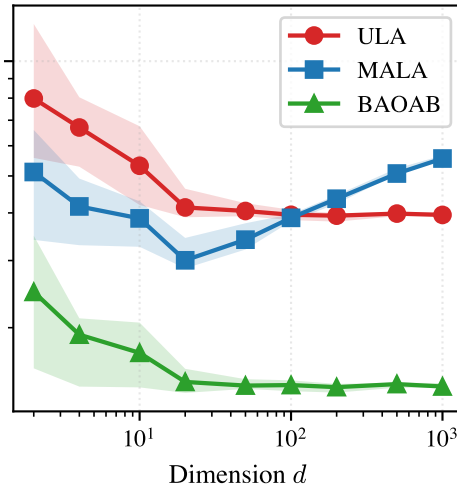
Anisotropic ( \kappa = 1000 )
