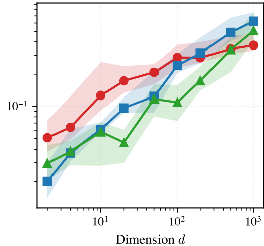
Funnel ( \sigma_v = 2 )
