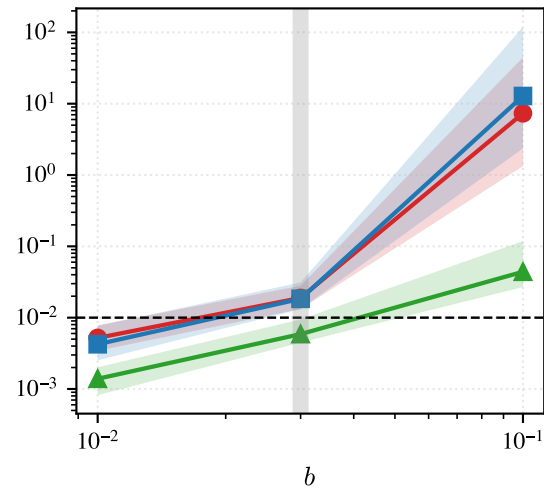
Banana
