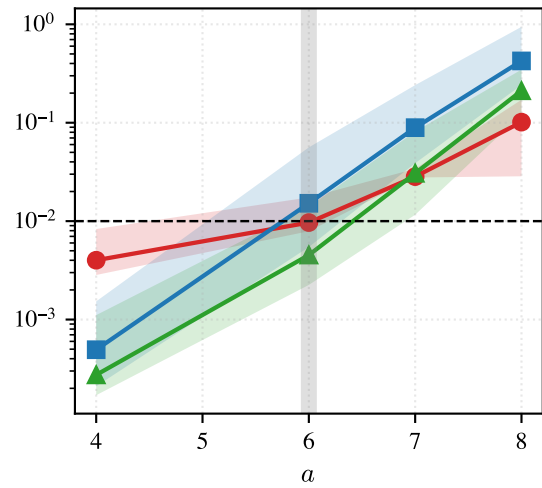
Mixture
