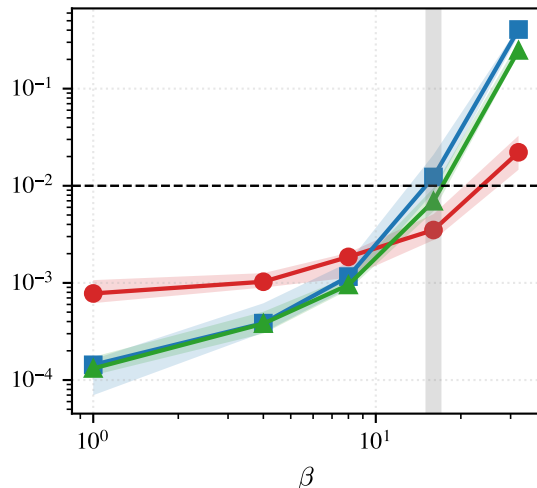
Double well
