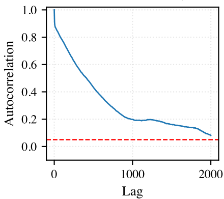
Autocorrelation of x_0
