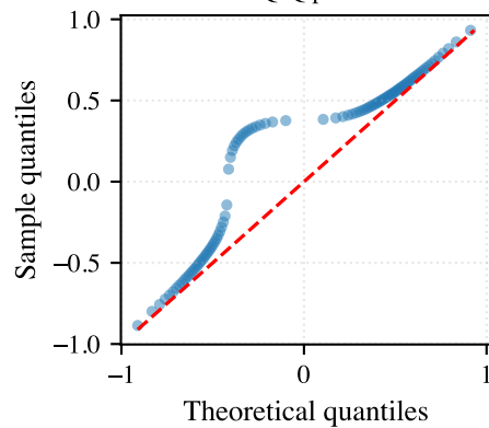
Q-Q plot
