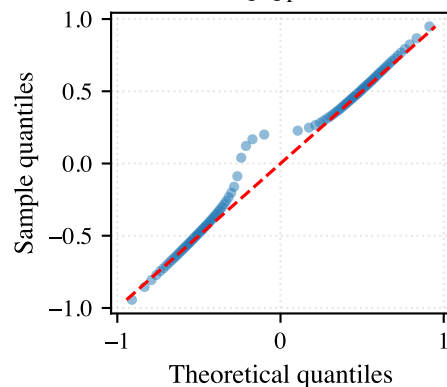
Q-Q plot
