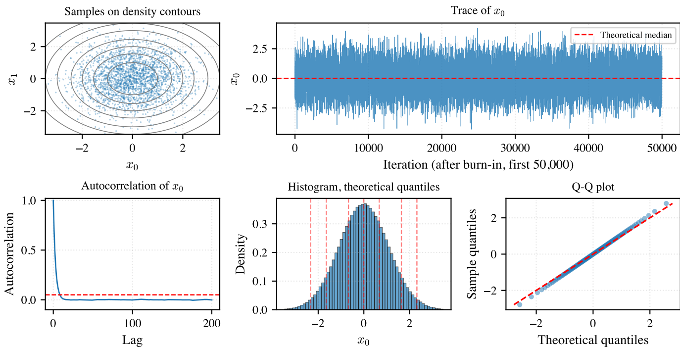
Gaussian, d = 10 . MALA ( \eta = 0.3 ), acceptance = 0.86, variance estimate = 1.000 (true 1)
