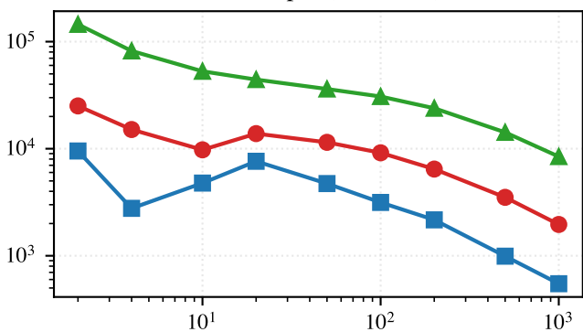
Mixture ( a = 6 )
