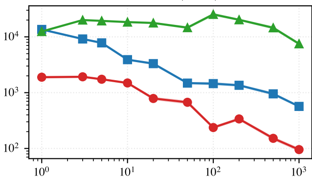
Anisotropic ( \kappa = 1000 )
