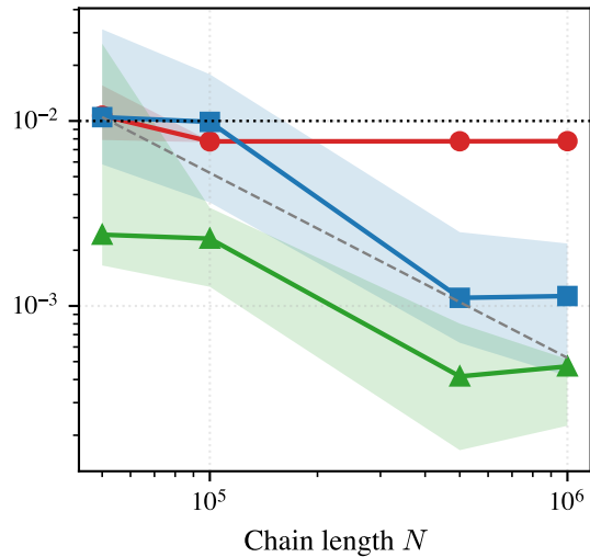
Mixture ( a = 6 )
