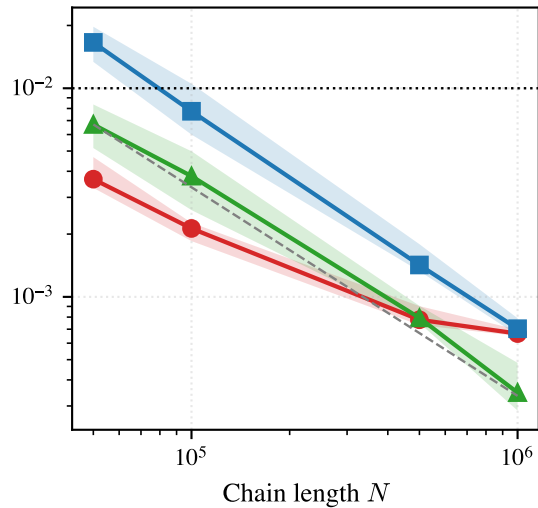
Double well ( \beta = 16 )
