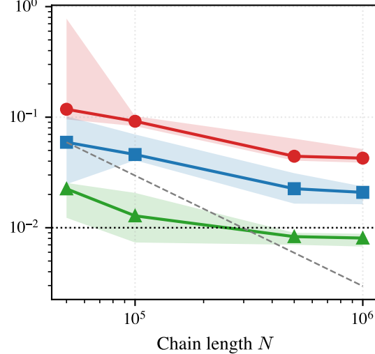
Funnel ( \sigma_v = 2 )
