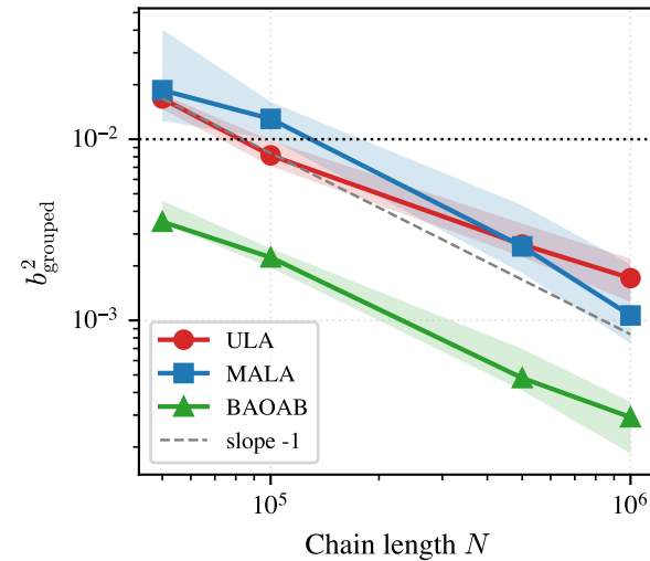
Banana ( b = 0.03 )
