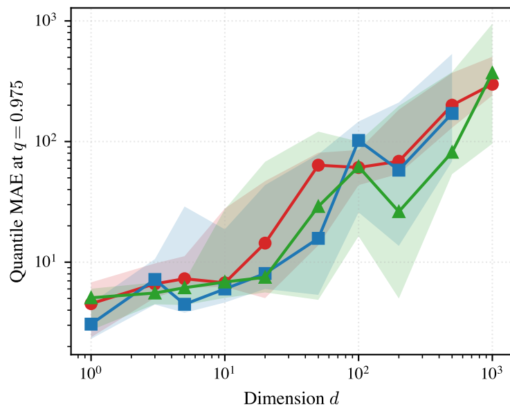
Cauchy diagnostics versus dimension (best configuration per d )
