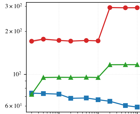
Double well ( \beta = 16 )
