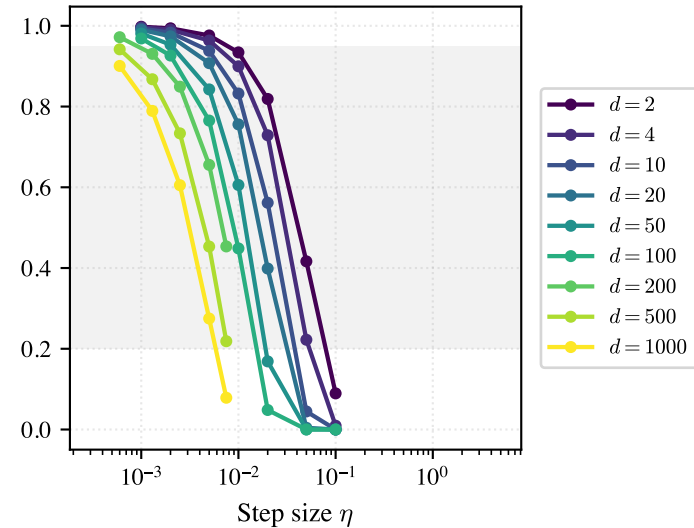
Double well ( \beta = 16 )
