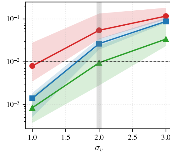
Funnel
