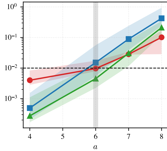
Mixture
