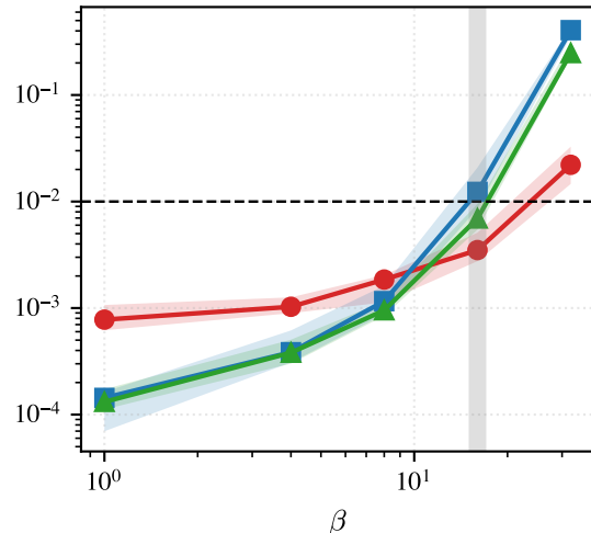
Double well
