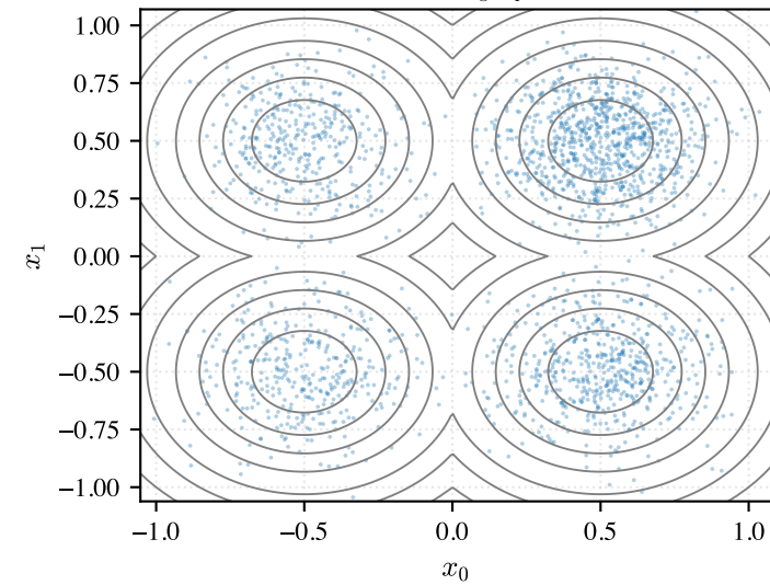
MALA ( \eta = 0.01 ), b_{\text{grouped}}^2 = 0.0123
