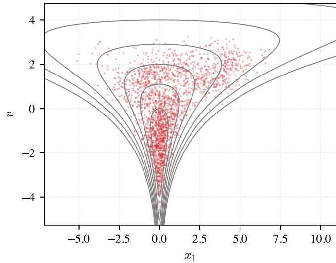
ULA ( \eta = 0.005 ), b_{\text{grouped}}^2 = 0.0545
