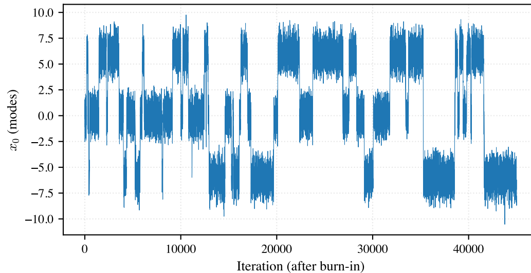
Trace of x_0 (modes)
