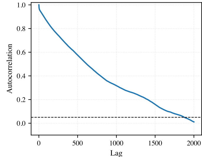
Autocorrelation of x_0 (modes)
