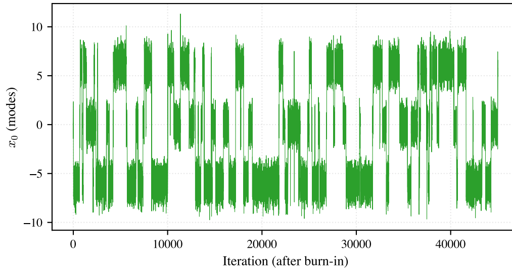
Trace of x_0 (modes)
