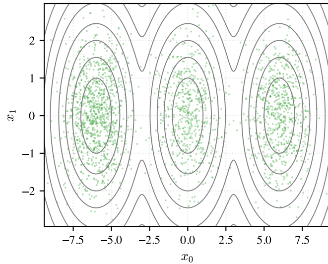
MALA ( \eta = 0.3 ), b_{\text{grouped}}^2 = 0.0152
