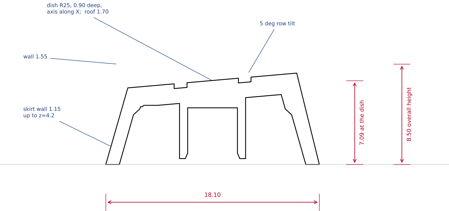
C SECTION X = 0 (side, front of the keyboard to the left) OEM-style sculpt: top plate tilted back, cylindrical dish
