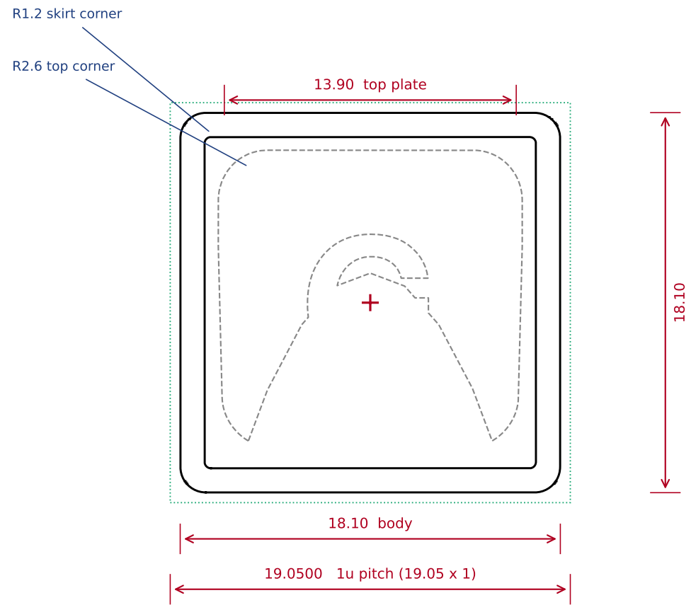
A PLAN (top) outline at the skirt and at the top plate
