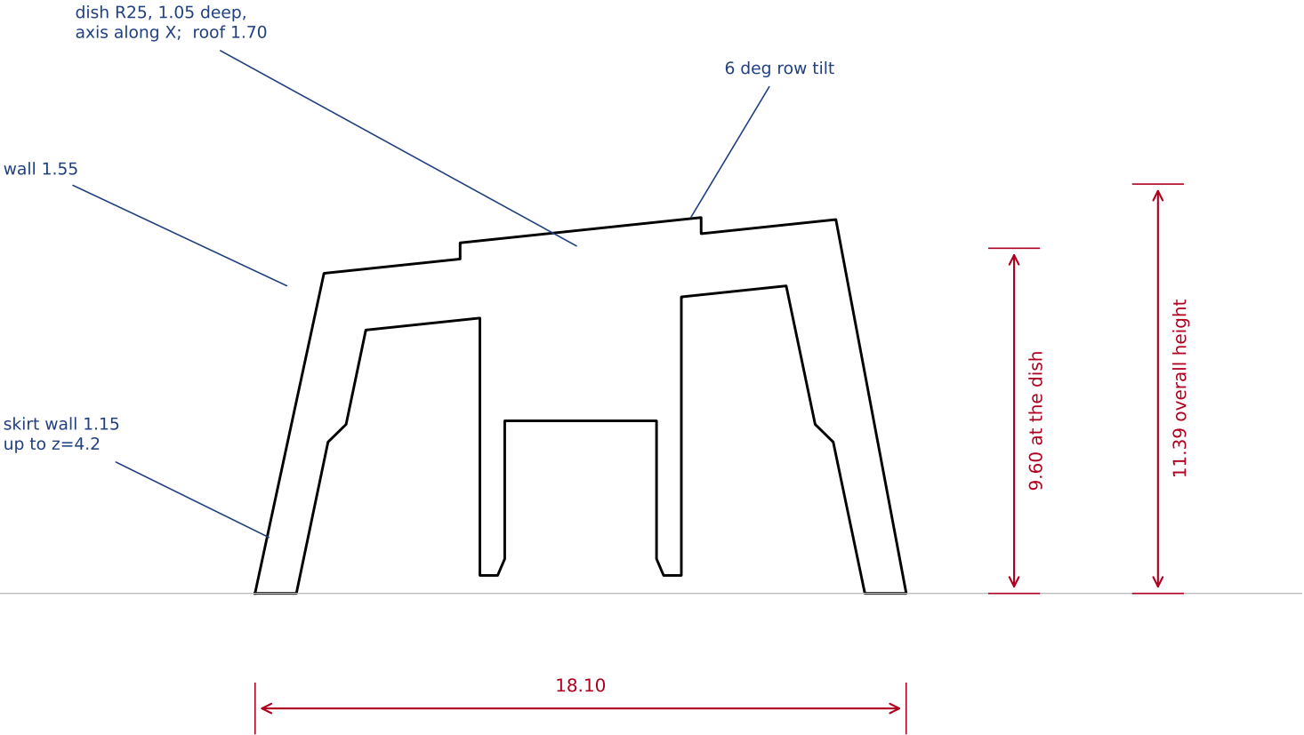
C SECTION X = 0 (side, front of the keyboard to the left) OEM-style sculpt: top plate tilted back, cylindrical dish
