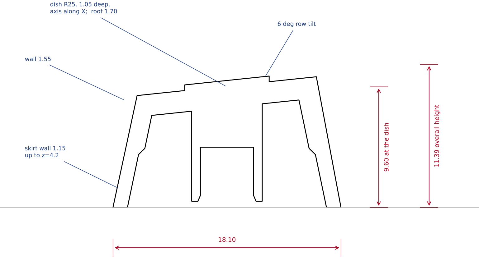
C SECTION X = 0 (side, front of the keyboard to the left) OEM-style sculpt: top plate tilted back, cylindrical dish
