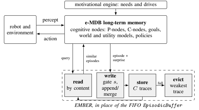
Fig. 1. Where EMBER would sit in e-MDB (schematic; not implemented here). e-MDB activates cognitive nodes in its long-term memory from the current perception and selects actions under its motivational engine [1], [32]; each step yields an Episode that the public implementation appends to a FIFO EpisodicBuffer from which world and utility models are trained [3]. EMBER would replace that buffer: write weights each episode by a surprise signal supplied by e-MDB’s own world or utility models, evict discards the weakest trace when the store is full, and read returns the stored episodes most similar to a query, feeding model training and deliberation.
