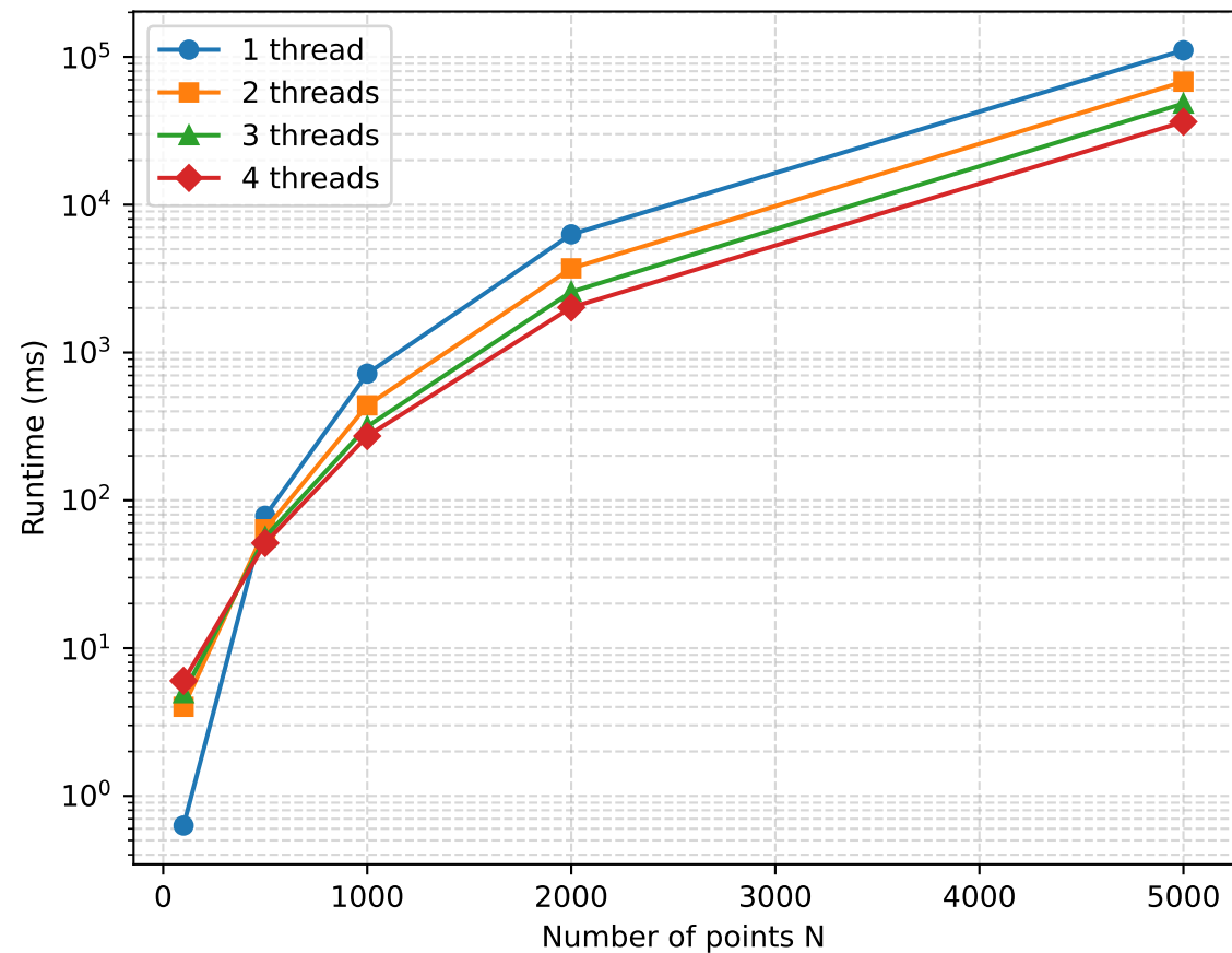
Runtime vs Dataset Size
