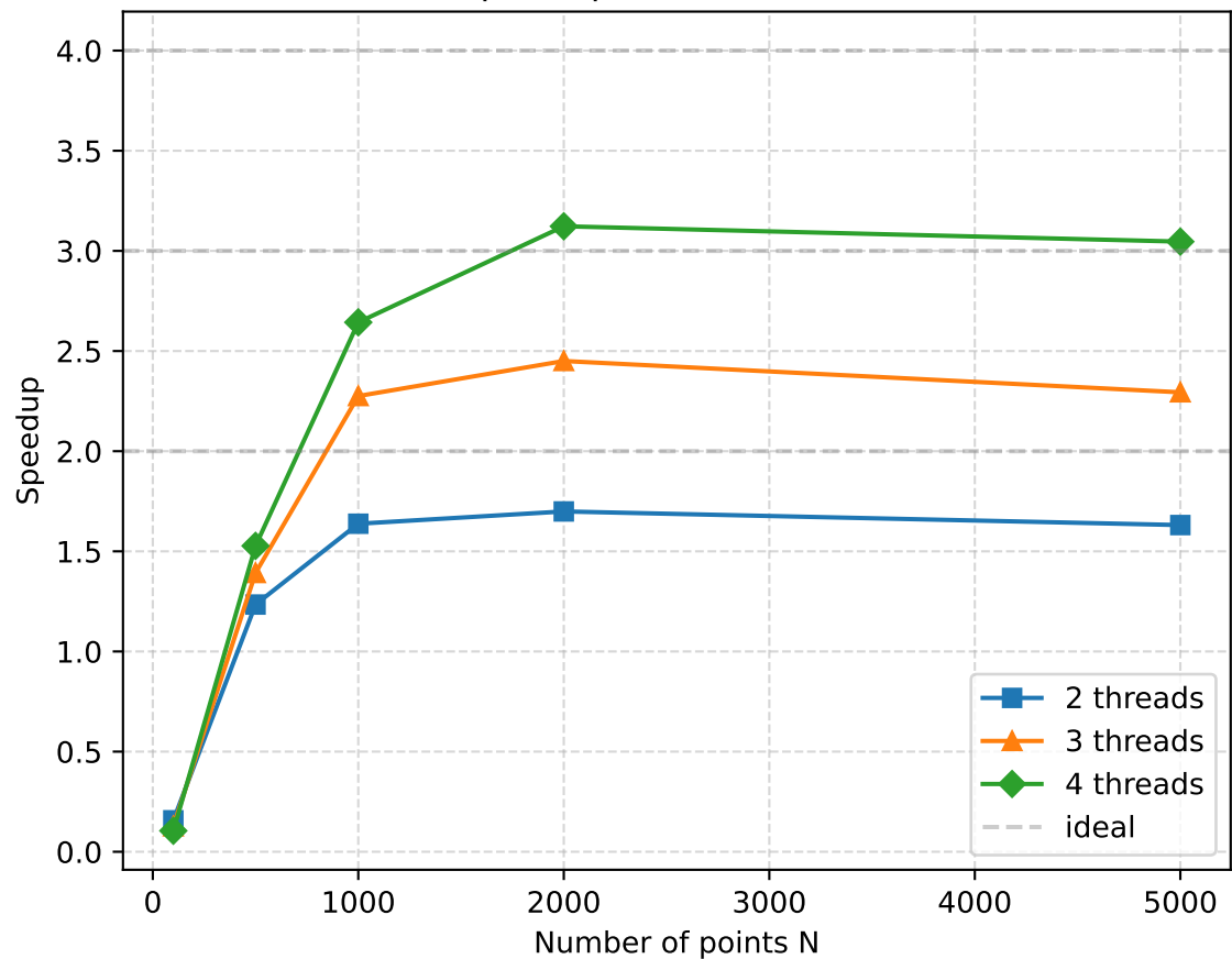
Speedup vs Dataset Size
