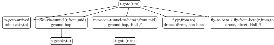
Figure 2: t-goto five methods
