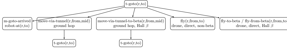
Figure 2: t-goto ’s five methods. Recursion (the two ”hop, then recurse” ground methods) terminates within two levels since the map is a radius-1 star around the Maintenance Tunnel; the three drone methods never need to recurse at all, since a flight is always a single hop.
