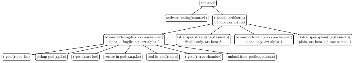
Figure 1: Problem 3 task hierarchy, t-mission down to primitive actions, with the alpha+fragile branch ( art-alpha-2 ) expanded in full. The other three t-handle-artifact methods follow the same pod/direct \times cool/no-cool shape (Table 3).
