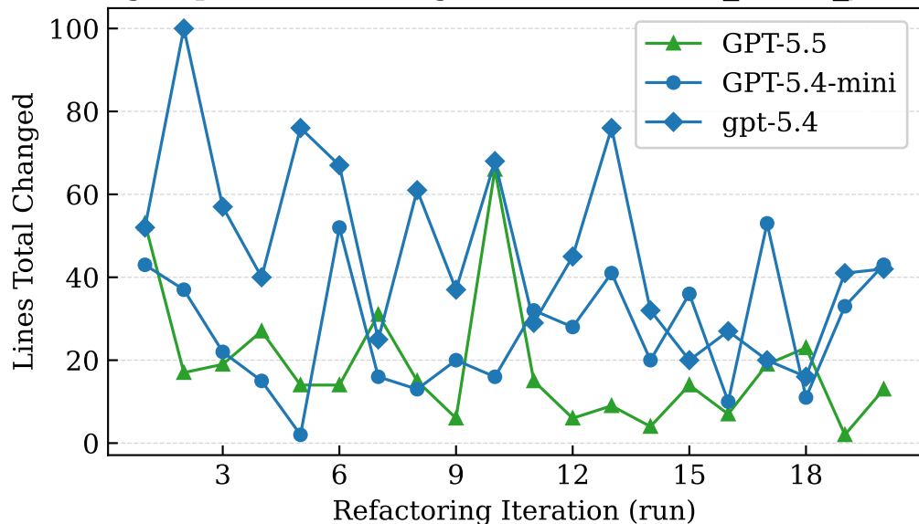
Lines Changed per Refactoring Run — BUBBLE_SORT_JAVA-TEMP0.0
